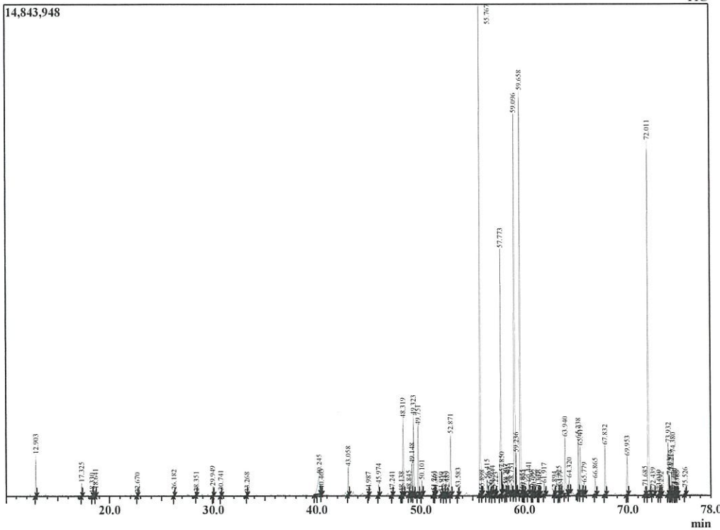
Chromatogram Callitris intratropica
