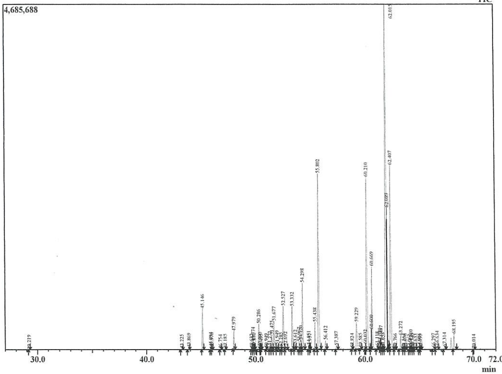
Chromatogram Amyris balsamifera
